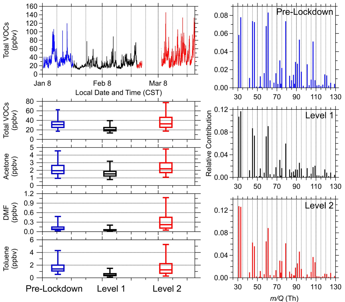
Figure 1. Time series for the total measured volatile organic compounds (VOCs) during the pre-lockdown (blue), level 1 (black), and level 2 (red) periods and their respective average mass spectra. Box-plots are also shown for total measured VOCs and a few select VOCs (whiskers are the 5th and 95th percentiles).
